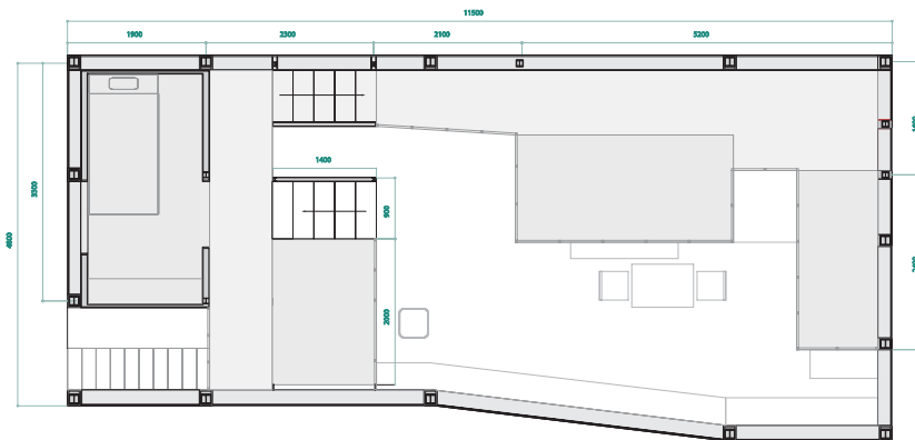
First Floor 1/150
