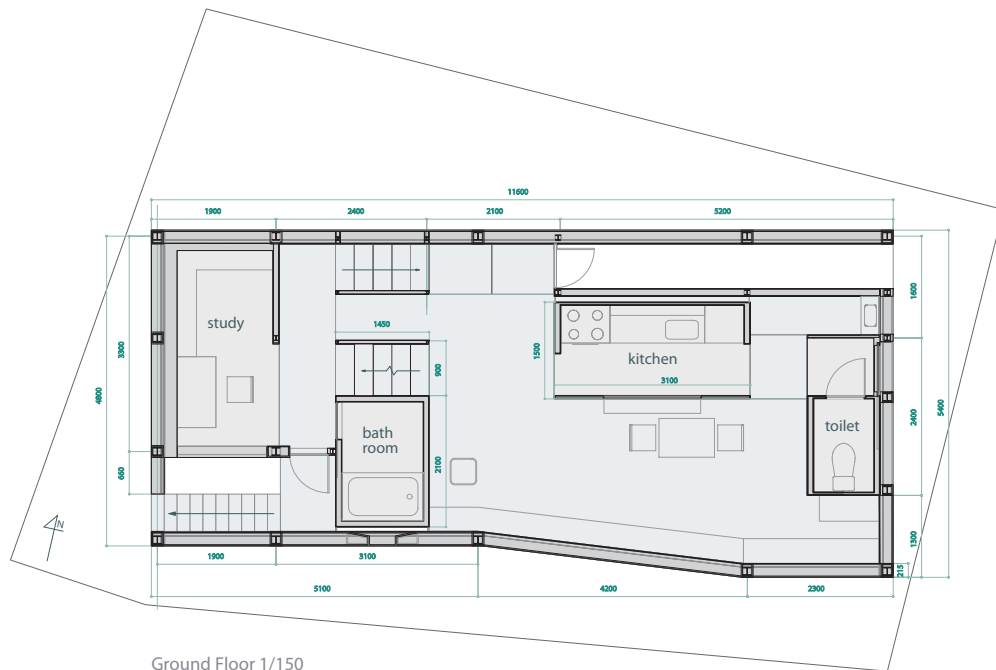
Ground Floor 1/150
